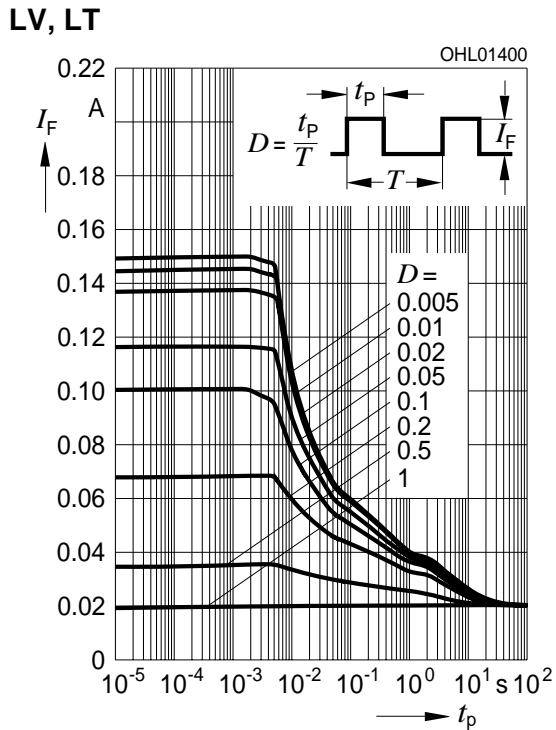
Zulässige Impulsbelastbarkeit I_F = f(t_p) Permissible Pulse Handling Capability Duty cycle D = \text{parameter} , T_A = 25\text{ °C}
