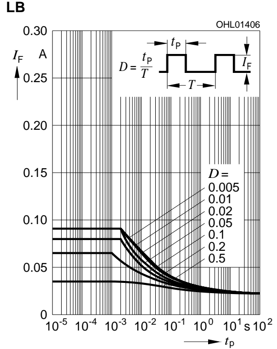
Zulässige Impulsbelastbarkeit I_F = f(t_p) Permissible Pulse Handling Capability Duty cycle D = \text{parameter} , T_A = 85\text{ °C}
